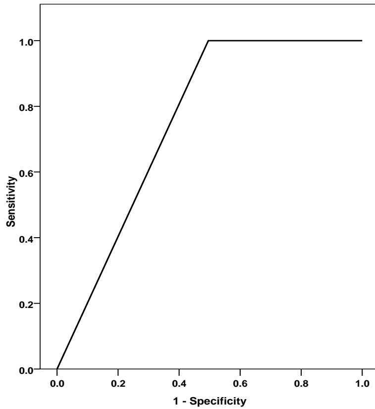
Fig. (4): showing AUC for serum ficolin-2 level as predictor for severe PE
