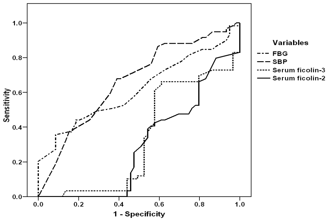
Fig. (2): showing ROC curve for studied variables as predictors for development of PE
