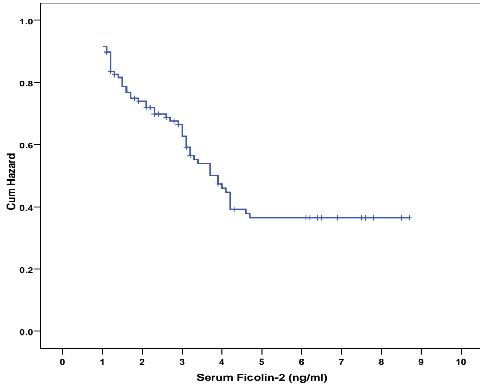
Fig. (3): showing cumulative hazard for developing PE at cutoff point for serum ficolin-2 of 4.793 ng/ml
